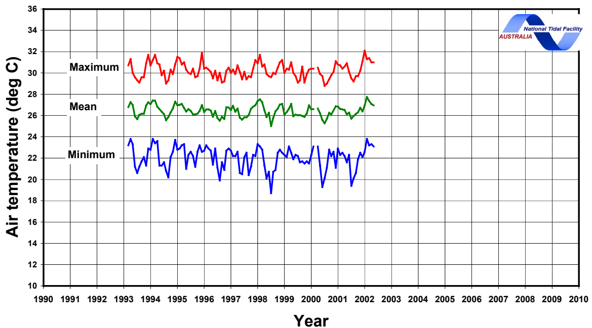
Monthly air temperature at Apia SEAFRAME gauge
