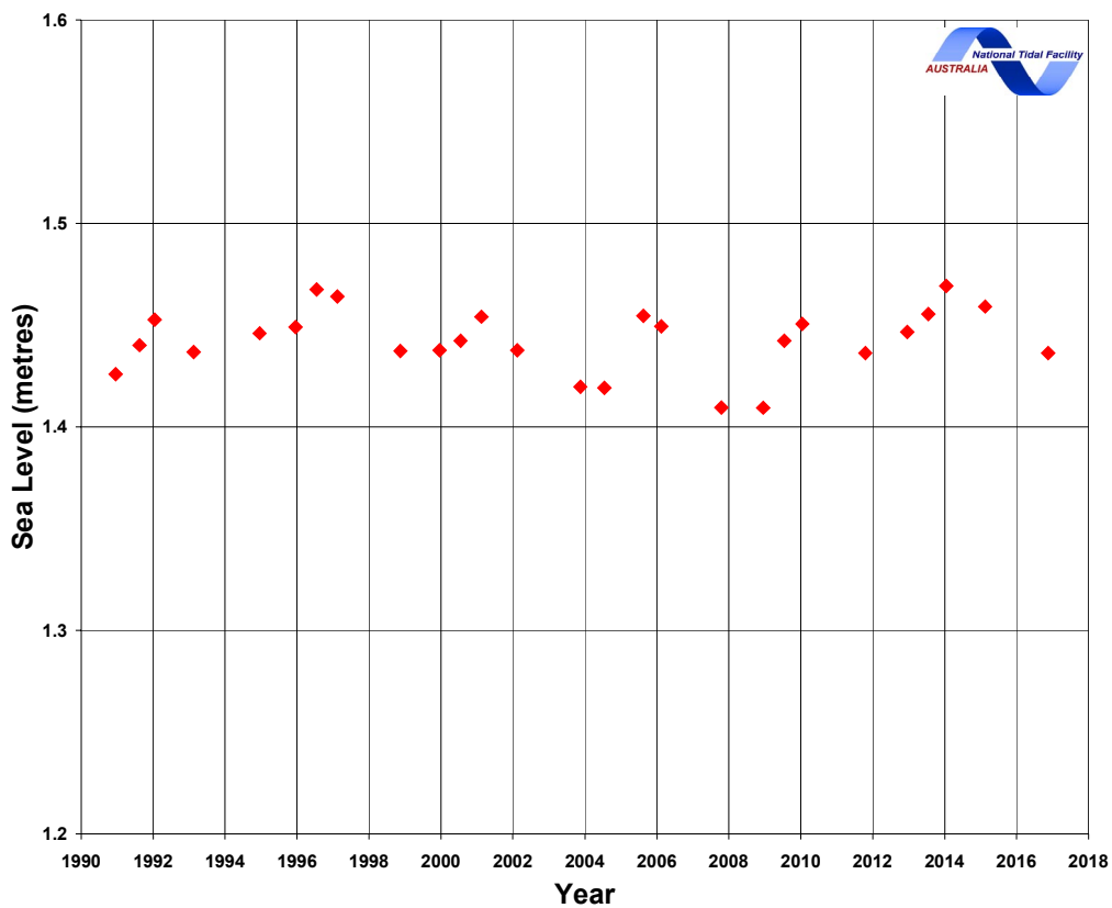
Predicted highest tide each year for Apia
