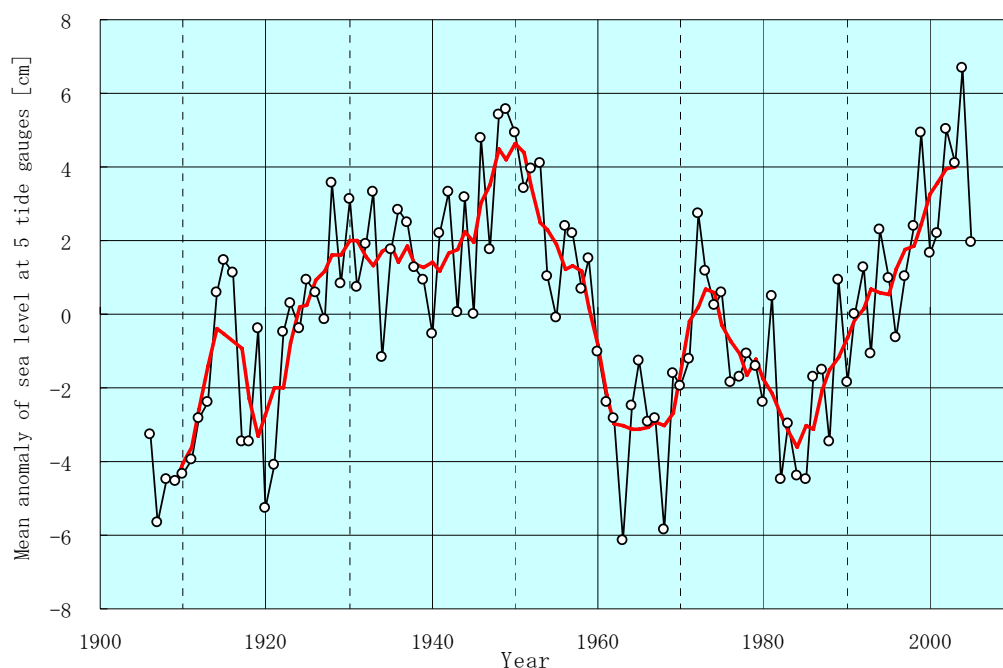
Fig. 2: Variations of anomaly of the annual mean sea levels from 100-year mean (average for 5 tide stations). Red line shows the 5-year running mean over the past 100 years.
